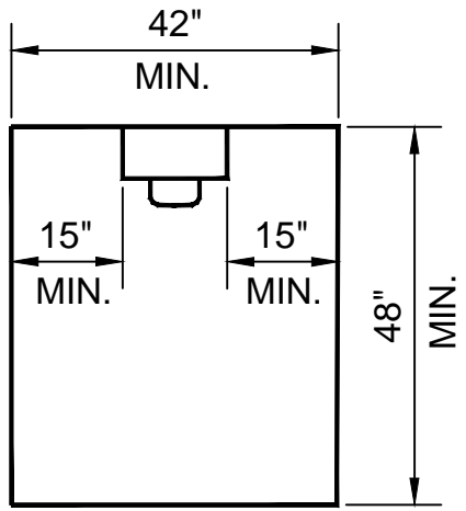
LANDING PLAN (MINIMUM CLEARANCES)
